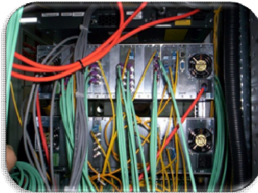
Installation of CWDM Fiber Module at Astro Measat Cyberjaya
